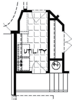
DROPPED GARAGE STAIRS OPTION
